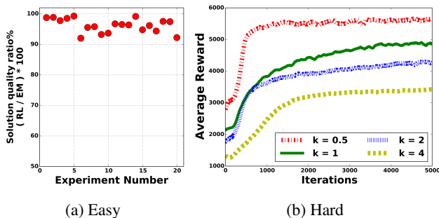
Figure 5: Solution Quality - Multiagent RL
