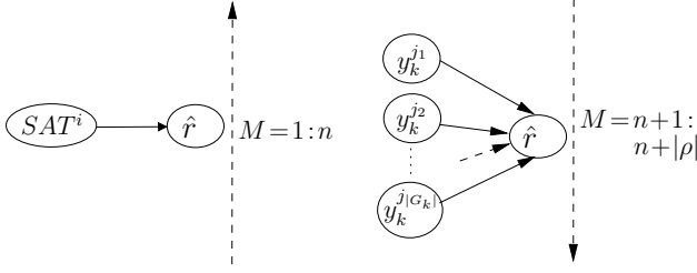
Figure 2: Mixture model for TIDec-MDP; M is mixture variable with discrete domain from 1 through n+|\rho| ; there is one BN (left) for each agent i=1:n ; one BN (right) for each joint-reward k \in \rho
